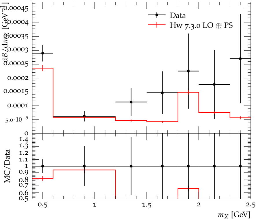
Mass distribution for X_s in B \rightarrow \eta' X_s
