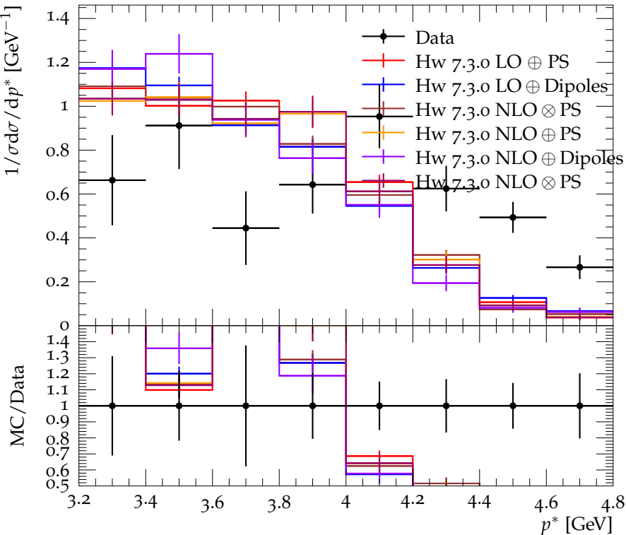
Momentum spectrum for D_{s1}(2460)^+ ( D_{s1}(2460)^+ \rightarrow D_S^+ \pi^0 \gamma )
