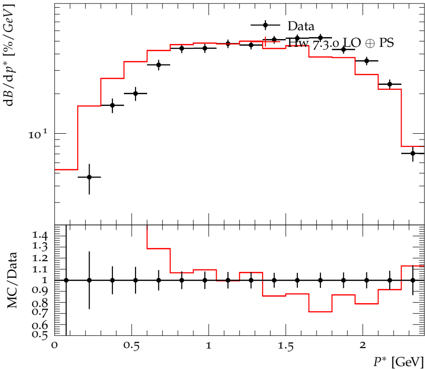
Branching ratio for B^- \rightarrow D^0 + X vs momentum
