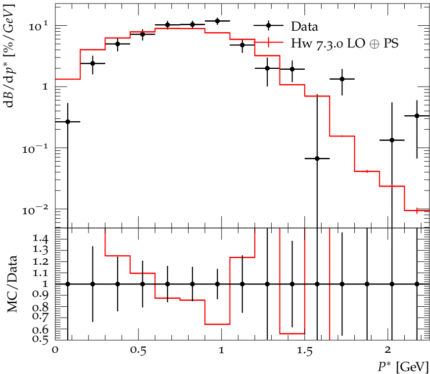
Branching ratio for B^- \rightarrow \bar{D}^0 + X vs momentum
