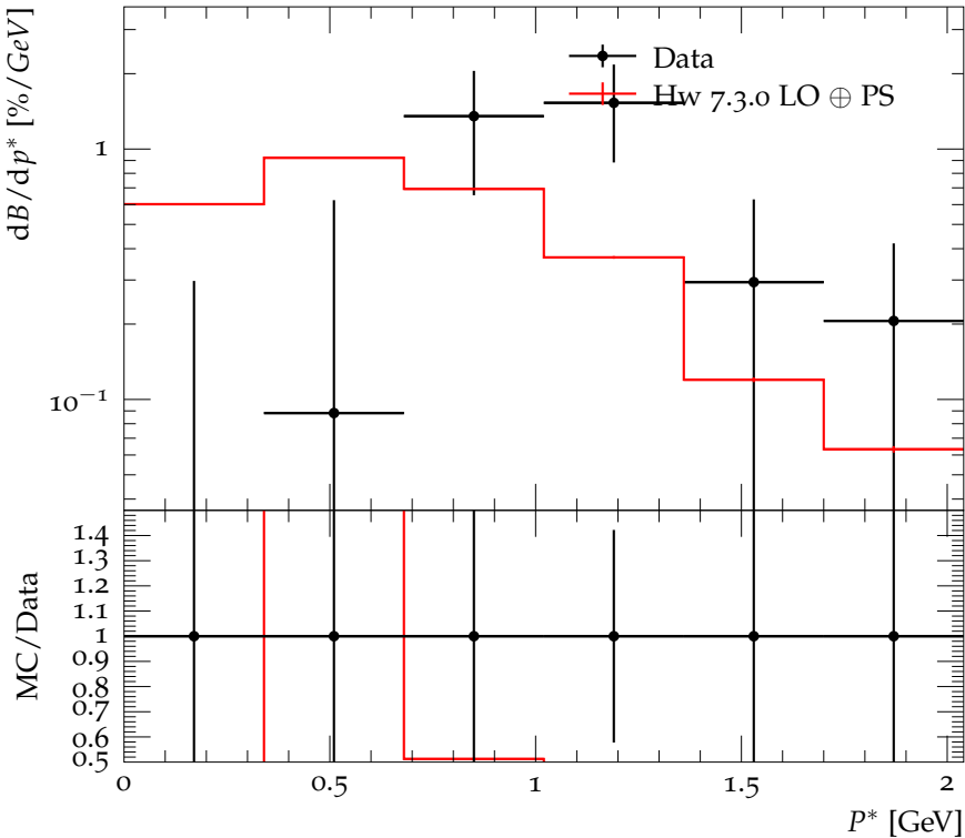
Branching ratio for B^- \rightarrow D_s^+ + X vs momentum
