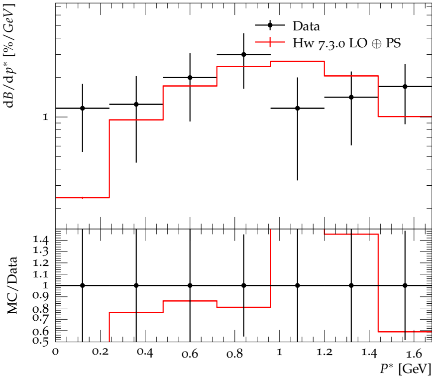
Branching ratio for B^- \rightarrow \Lambda_c^+ + X vs momentum
