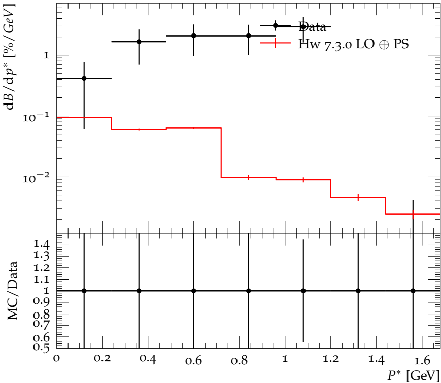
Branching ratio for B^- \rightarrow \bar{\Lambda}_c^- + X vs momentum
