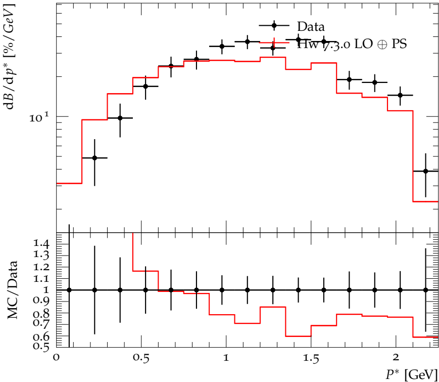
Branching ratio for \bar{B}^0 \rightarrow D^0 + X vs momentum
