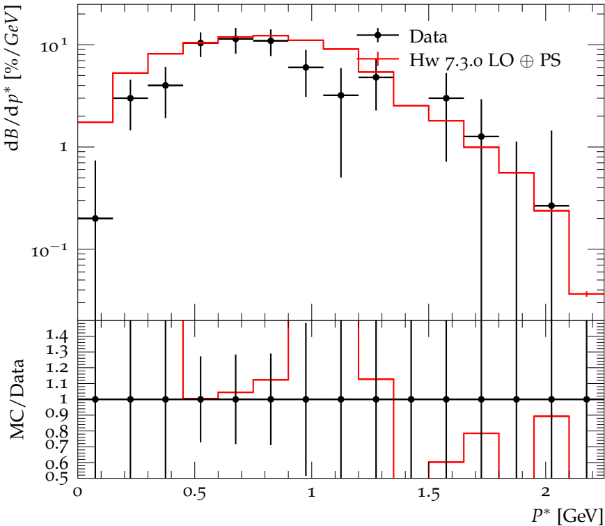
Branching ratio for \bar{B}^0 \rightarrow \bar{D}^0 + X vs momentum
