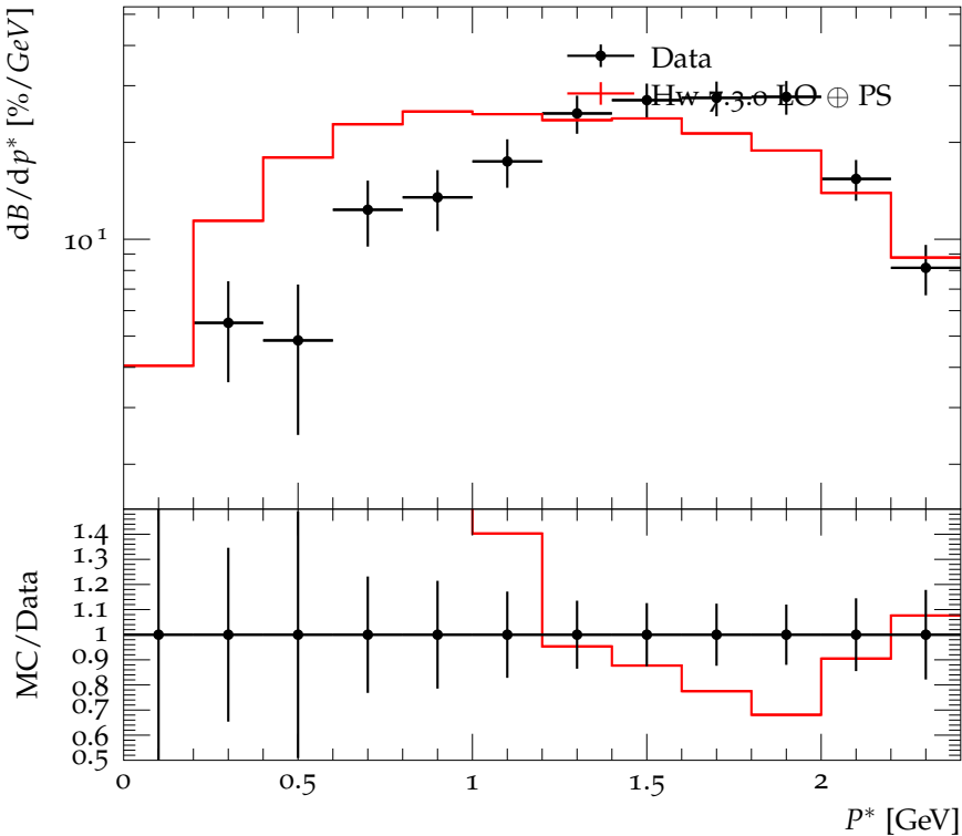
Branching ratio for \bar{B}^0 \rightarrow D^+ + X vs momentum
