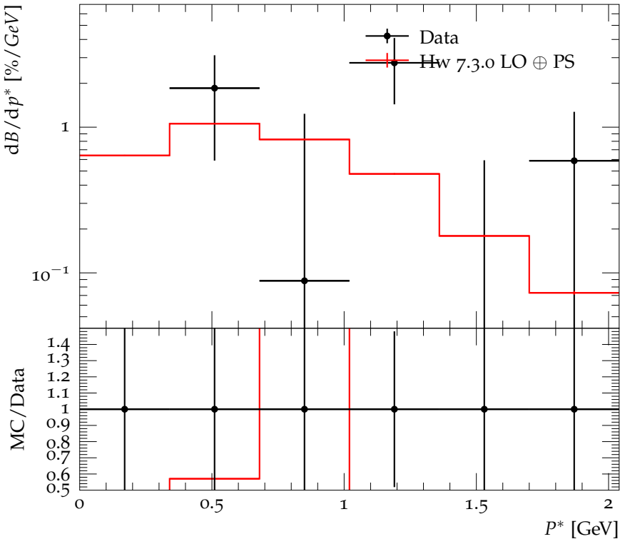
Branching ratio for \bar{B}^0 \rightarrow D_s^+ + X vs momentum
