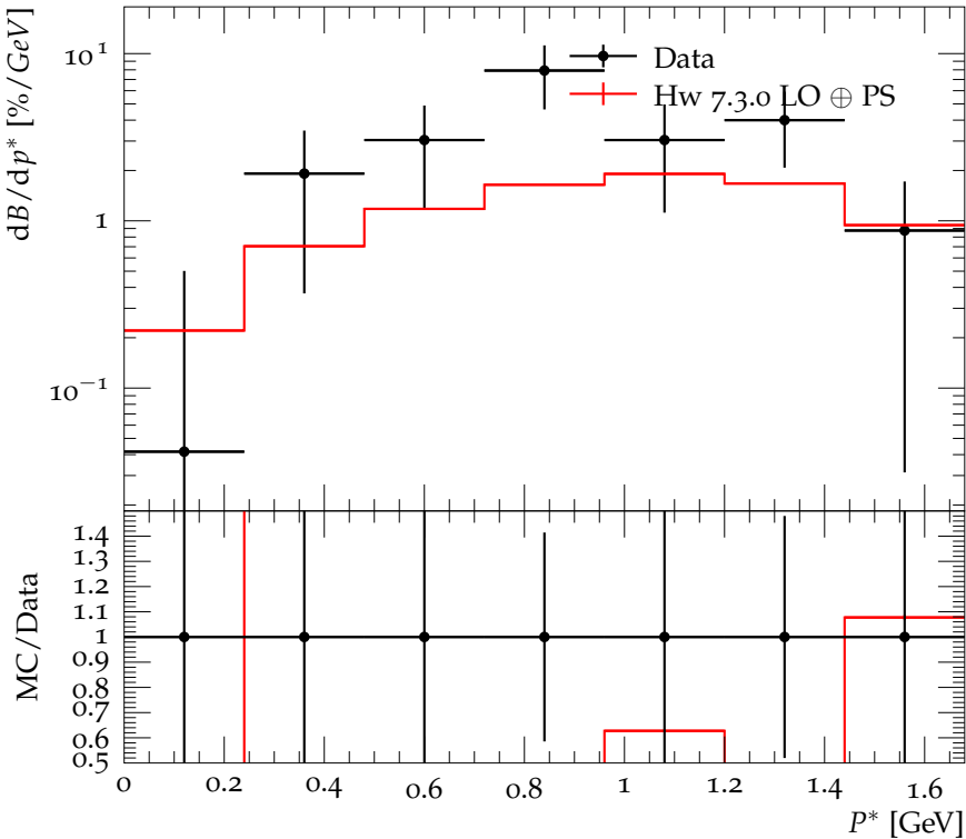
Branching ratio for \bar{B}^0 \rightarrow \Lambda_c^+ + X vs momentum
