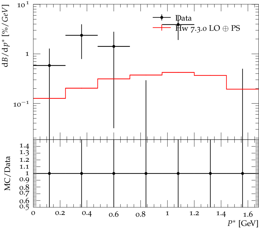
Branching ratio for \bar{B}^0 \rightarrow \bar{\Lambda}_c^- + X vs momentum
