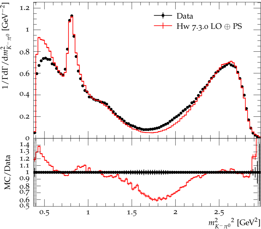
K^- \pi^0 mass distribution in D^0 \rightarrow K^- \pi^+ \pi^0
