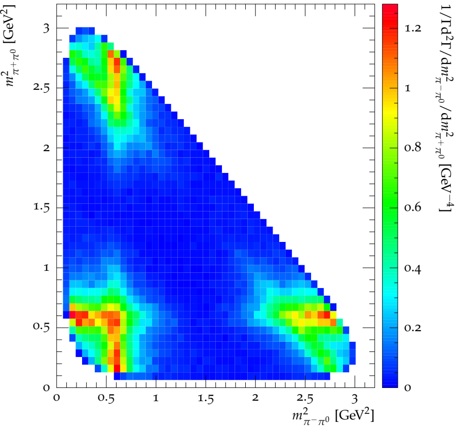
Dalitz plot for D^0 \rightarrow \pi^+ \pi^- \pi^0
