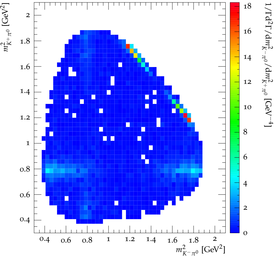
Dalitz plot for D^0 \rightarrow K^+K^-\pi^0
