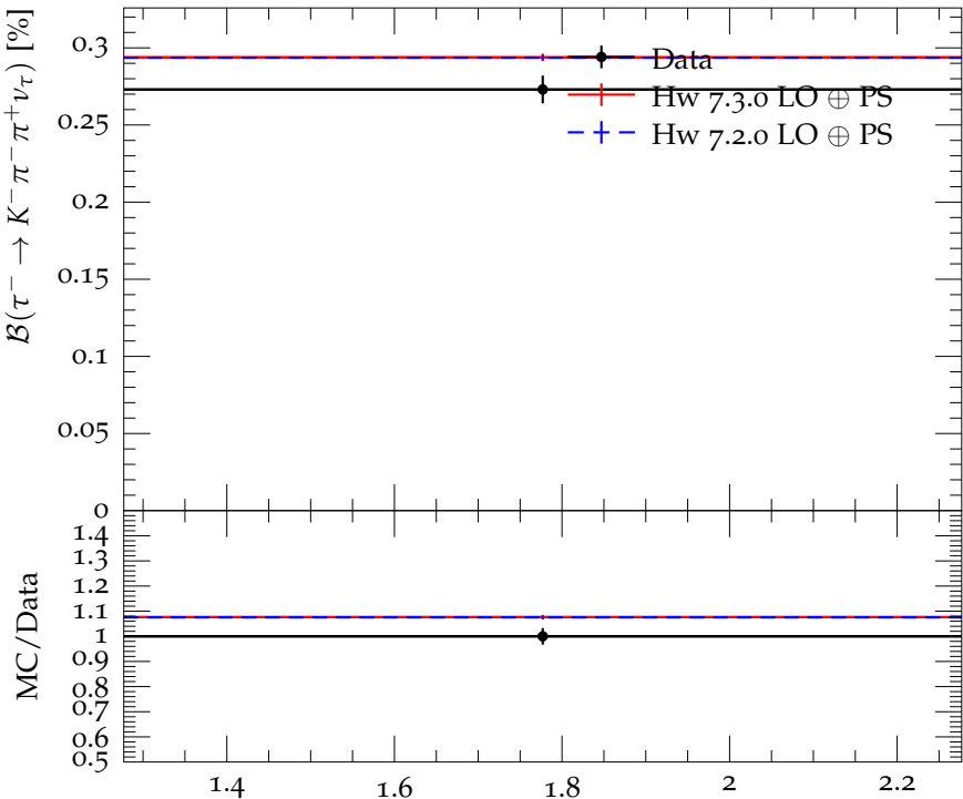
Branching ratio for \tau^- \rightarrow K^- \pi^- \pi^+ \nu_\tau decays
