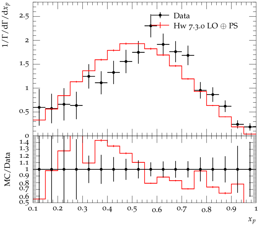
Spectrum of D^{*\pm} in Y(1S) decays
