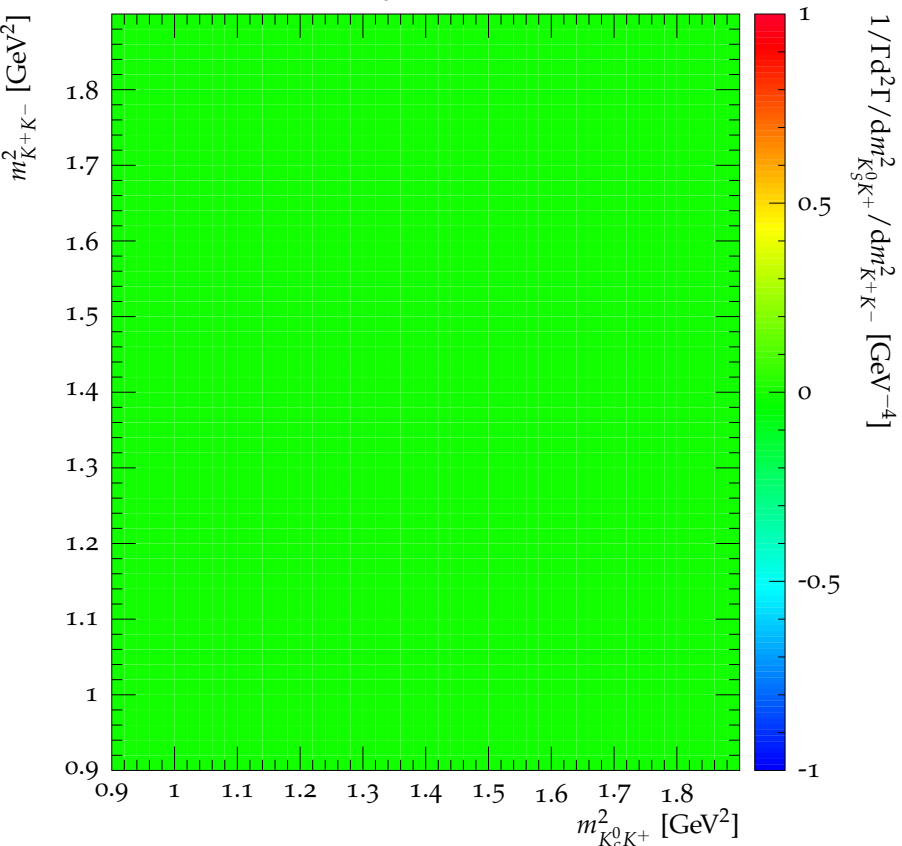
Dalitz plot for D^0 \rightarrow K_S^0 K^+ K^-
