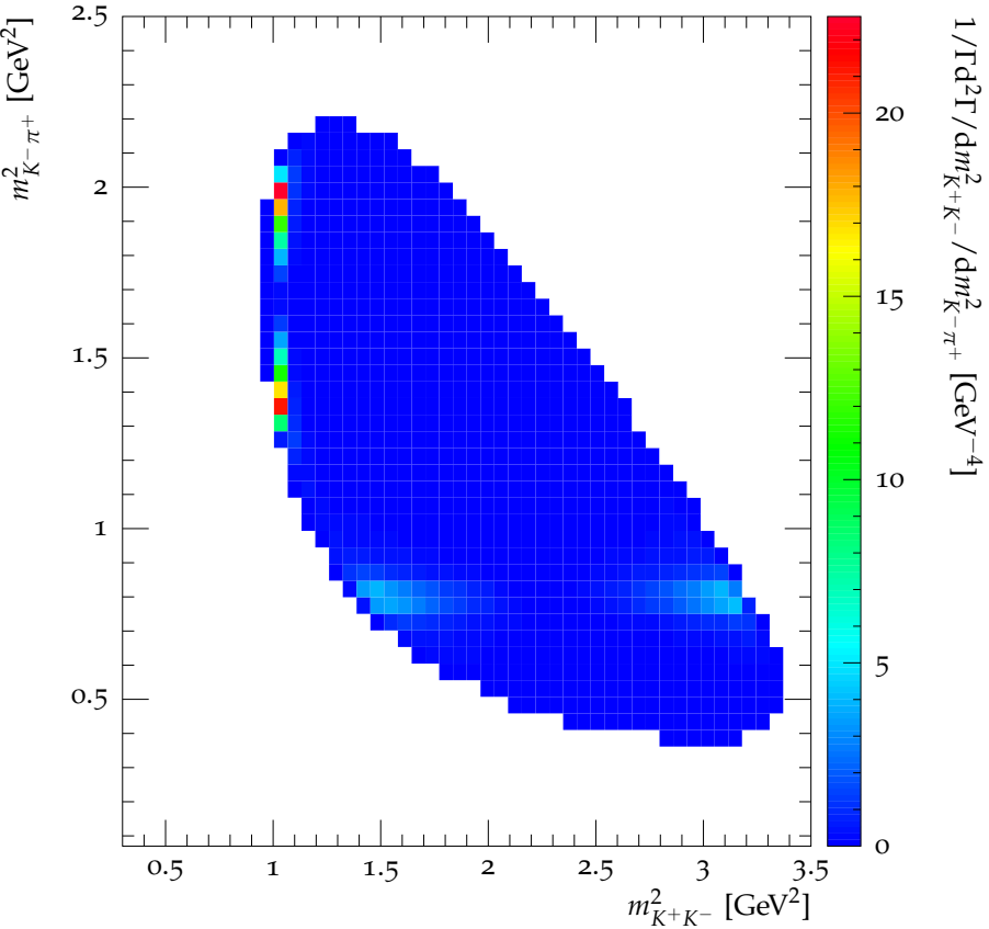
Dalitz plot for D_s^+ \rightarrow K^+ K^- \pi^+
