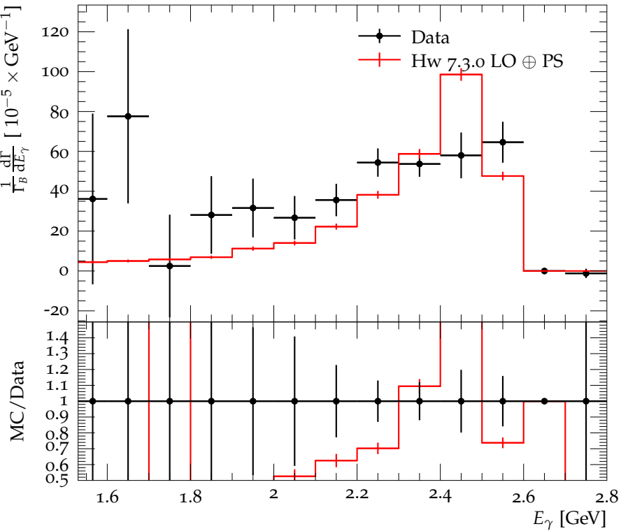
Photon energy spectrum for \bar{B} \rightarrow X_{s,d}\gamma
