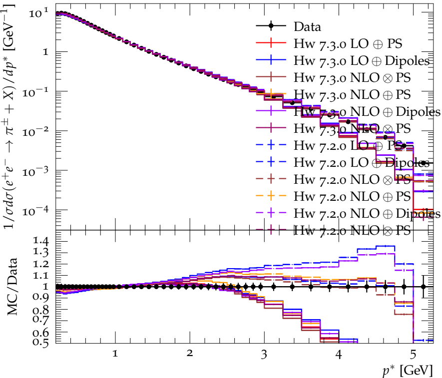
Spectrum for e^+e^- \rightarrow \pi^\pm + X including K_S and \Lambda decays
