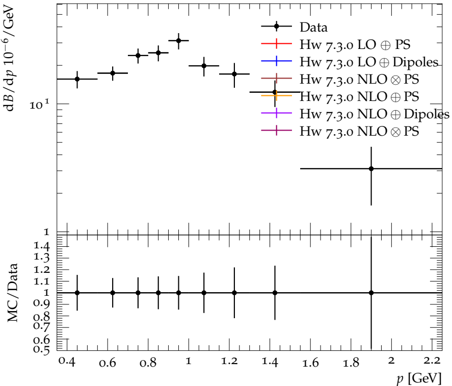
Momentum spectrum for anti-deuteron production in Y(2S) decay
