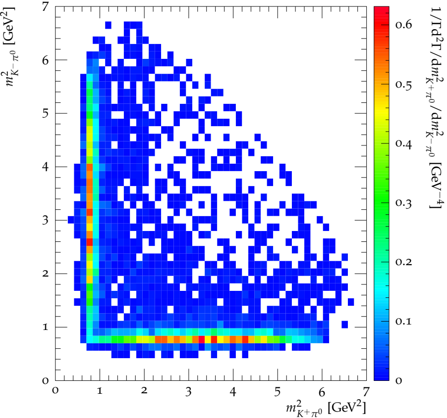
Dalitz plot for J/\psi \rightarrow K^+K^-\pi^0
