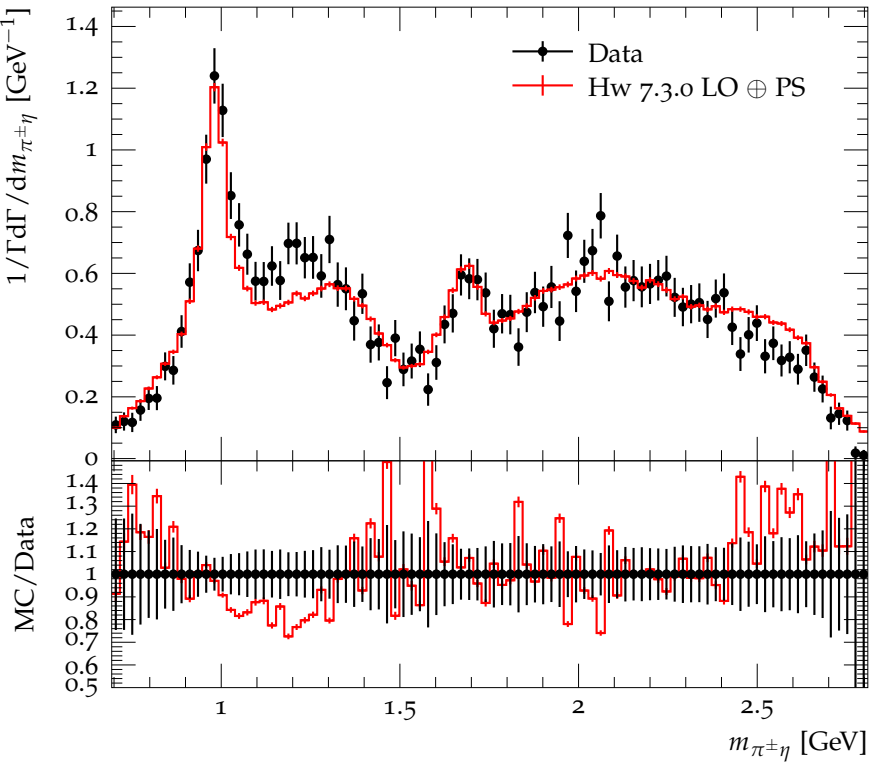
\pi^\pm\eta mass distribution in \eta_c \rightarrow \pi^+\pi^-\eta
