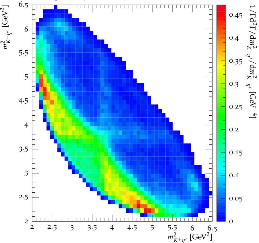
Dalitz plot for \eta_c \rightarrow K^+ K^- \eta'
