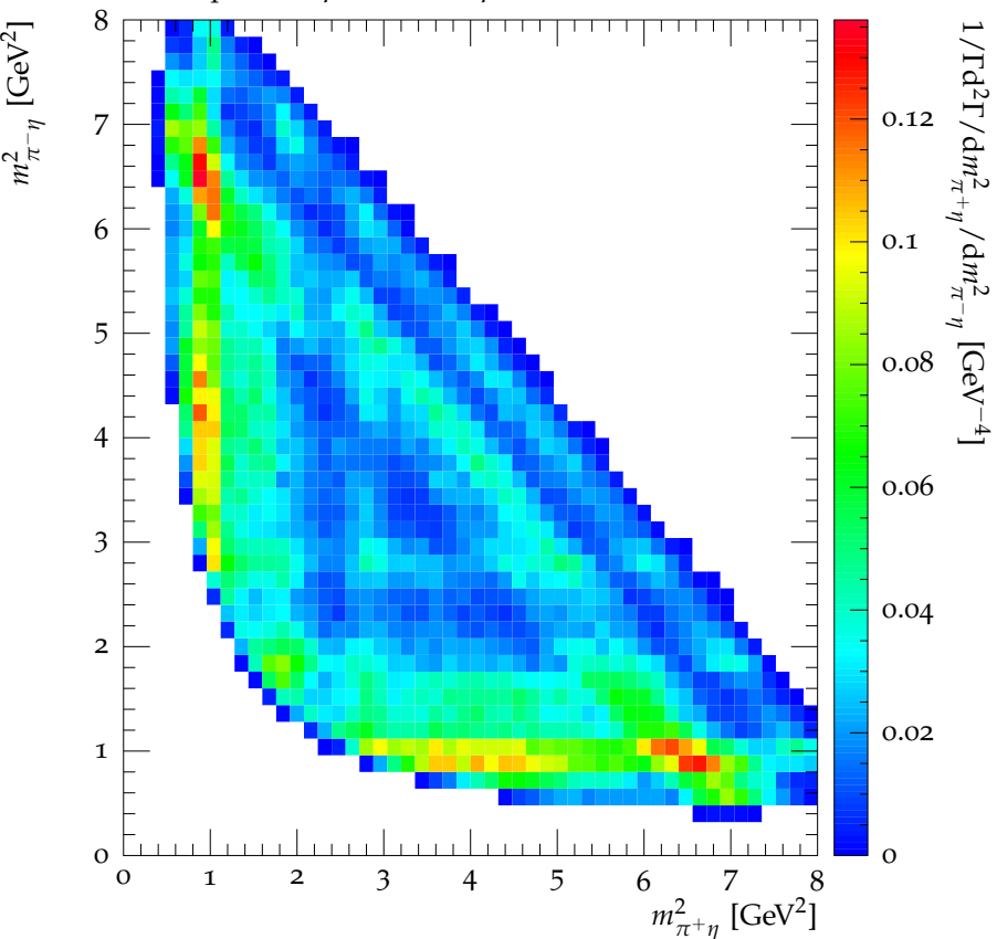
Dalitz plot for \eta_c \rightarrow \pi^+ \pi^- \eta
