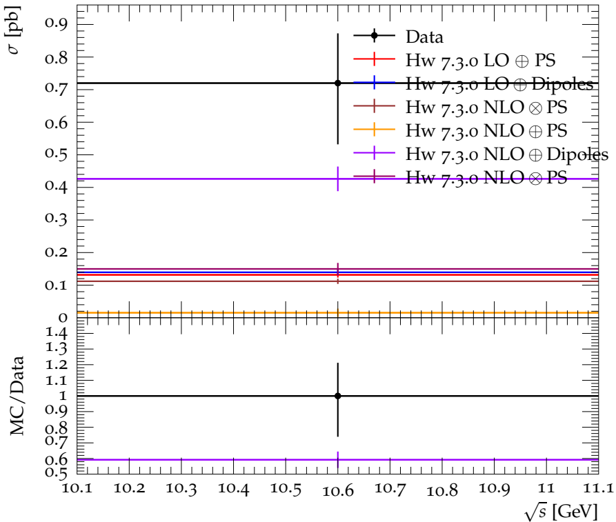
Cross Section for prompt J/\psi from \psi(2S) decay ( p^* > 2 GeV)
