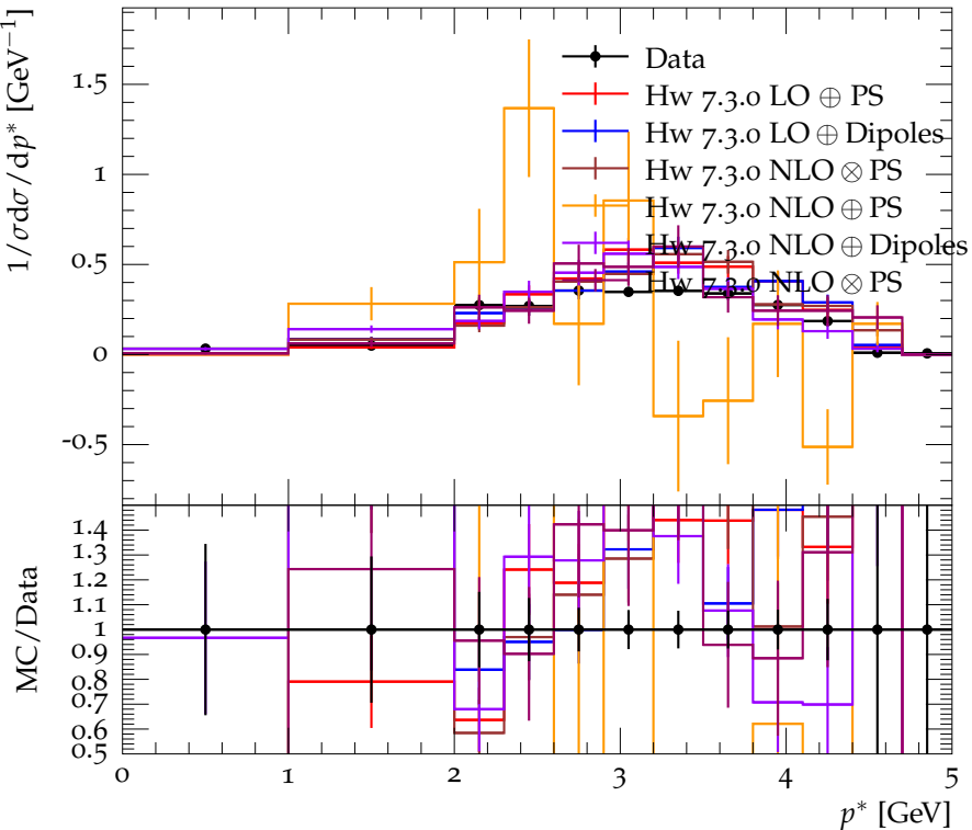
Spectrum for prompt J/\psi
