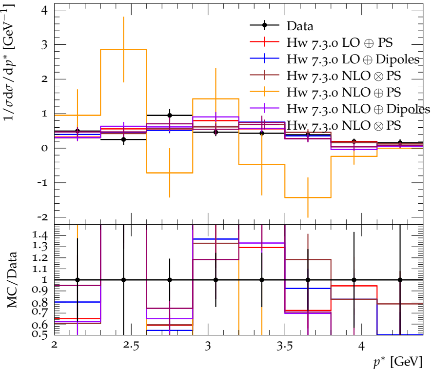
Spectrum for prompt J/\psi from \psi(2S) decay
