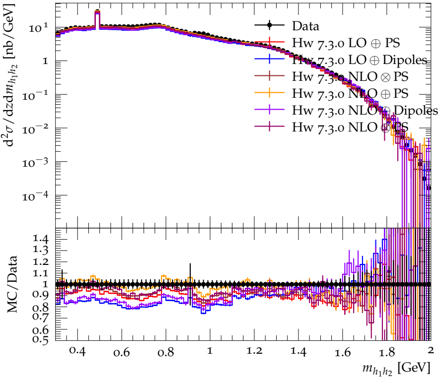
Differential cross section for \pi^+\pi^- ( 0.35 < z < 0.4 )
