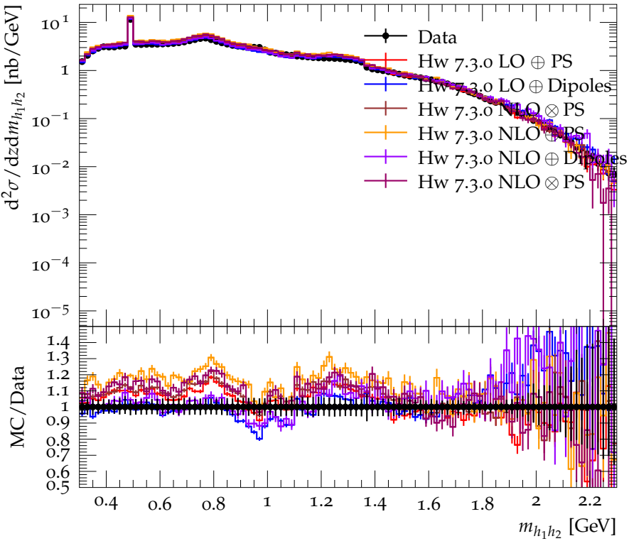
Differential cross section for \pi^+\pi^- ( 0.5 < z < 0.55 )
