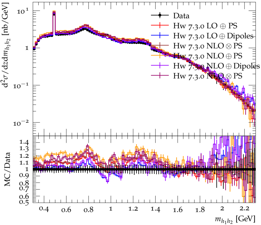
Differential cross section for \pi^+\pi^- ( 0.55 < z < 0.6 )
