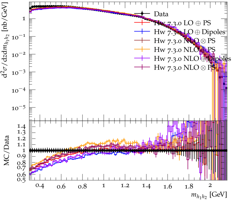
Differential cross section for \pi^+\pi^+ ( 0.4 < z < 0.45 )
