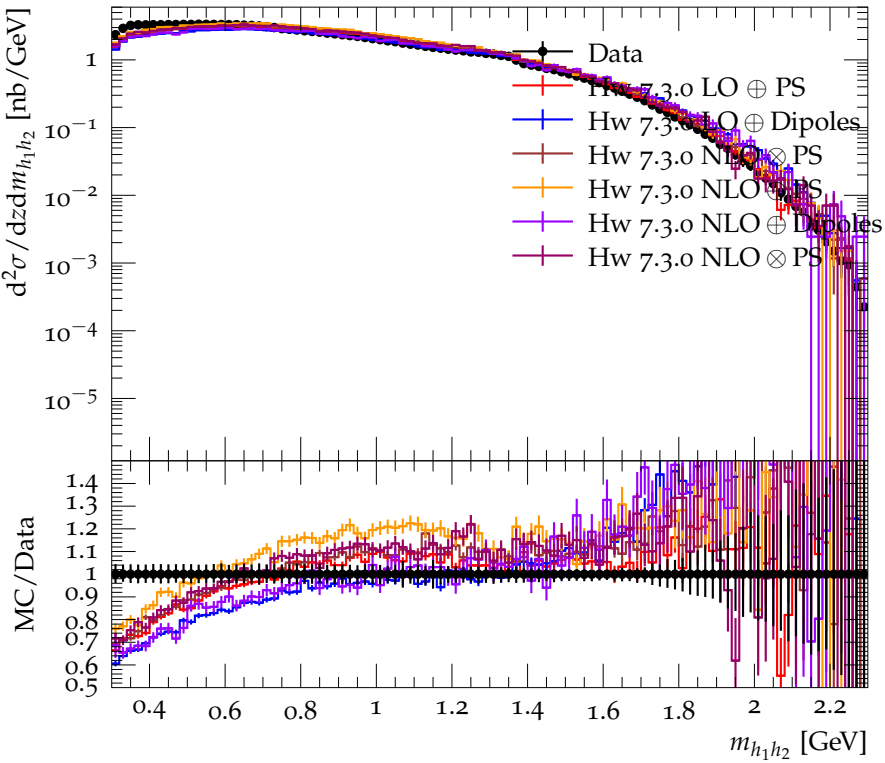
Differential cross section for \pi^+\pi^+ ( 0.45 < z < 0.5 )
