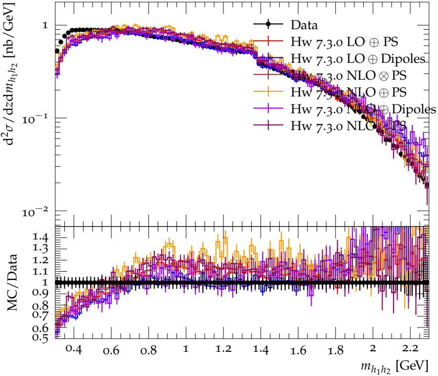
Differential cross section for \pi^+\pi^+ ( 0.6 < z < 0.65 )
