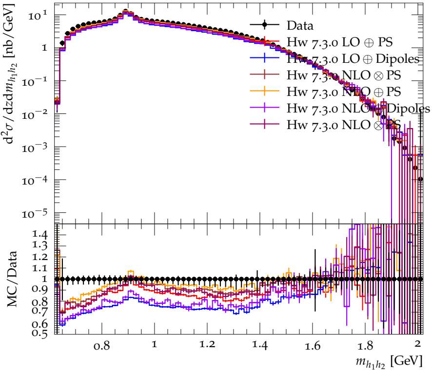
Differential cross section for \pi^+K^- ( 0.35 < z < 0.4 )
