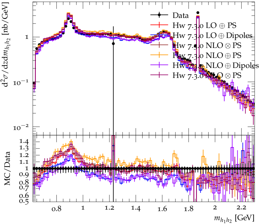
Differential cross section for \pi^+K^- ( 0.6 < z < 0.65 )
