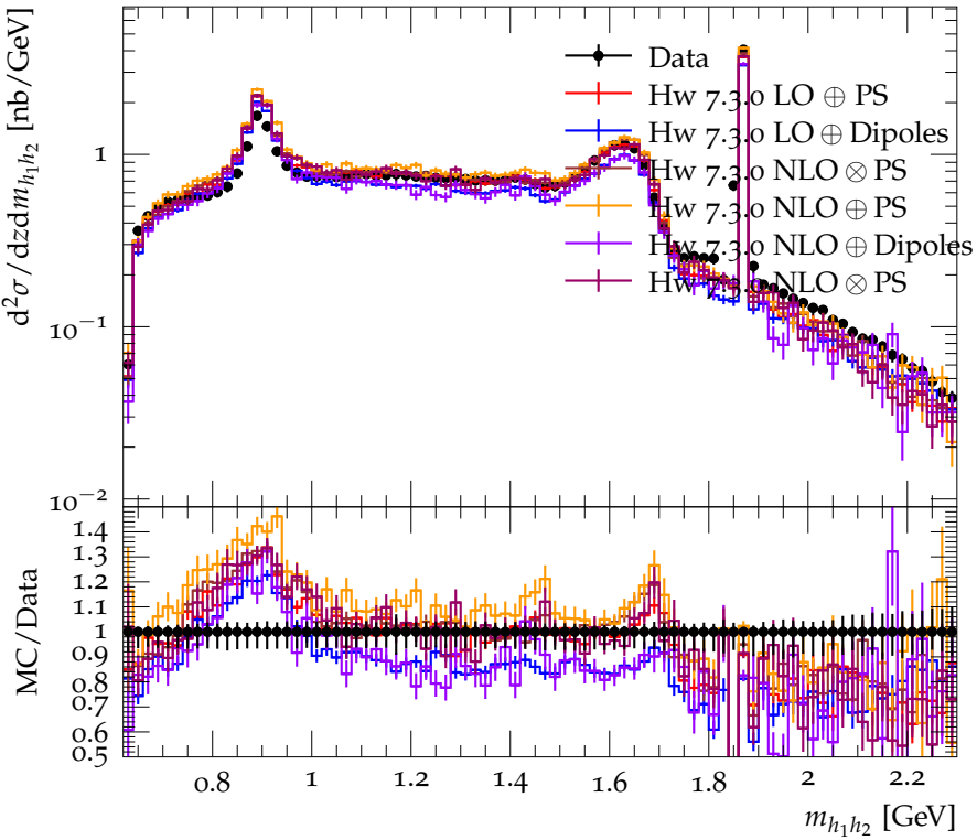
Differential cross section for \pi^+K^- ( 0.65 < z < 0.7 )
