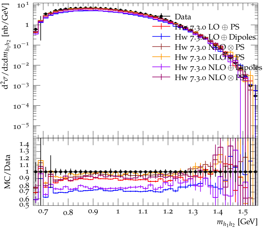
Differential cross section for \pi^+K^+ ( 0.25 < z < 0.3 )
