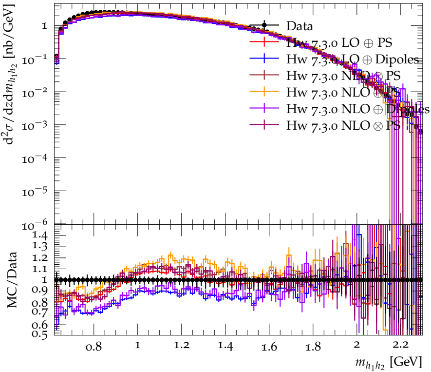
Differential cross section for \pi^+K^+ ( 0.45 < z < 0.5 )
