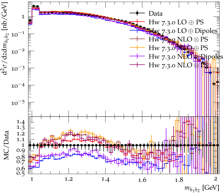
Differential cross section for K^+K^- ( 0.35 < z < 0.4 )
