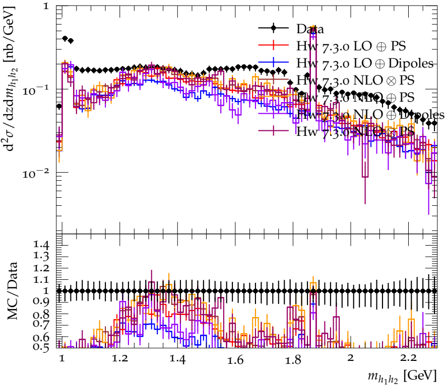
Differential cross section for K^+K^- ( 0.75 < z < 0.8 )
