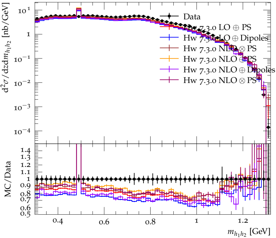
Differential cross section for \pi^+\pi^- ( 0.2 < z < 0.25 ) (strong)
