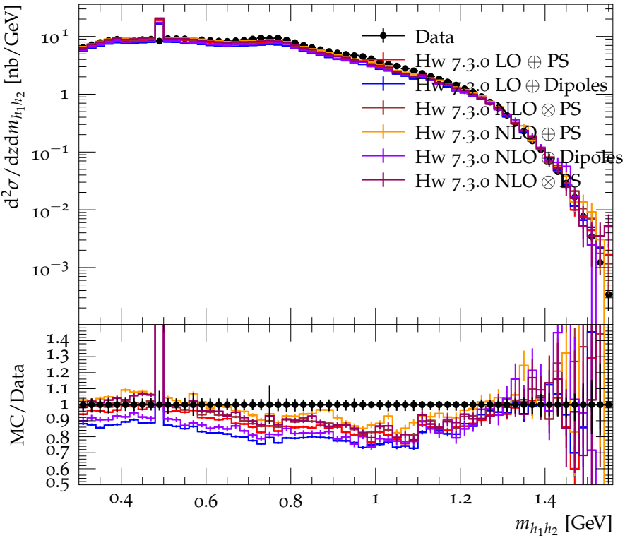
Differential cross section for \pi^+\pi^- ( 0.25 < z < 0.3 ) (strong)
