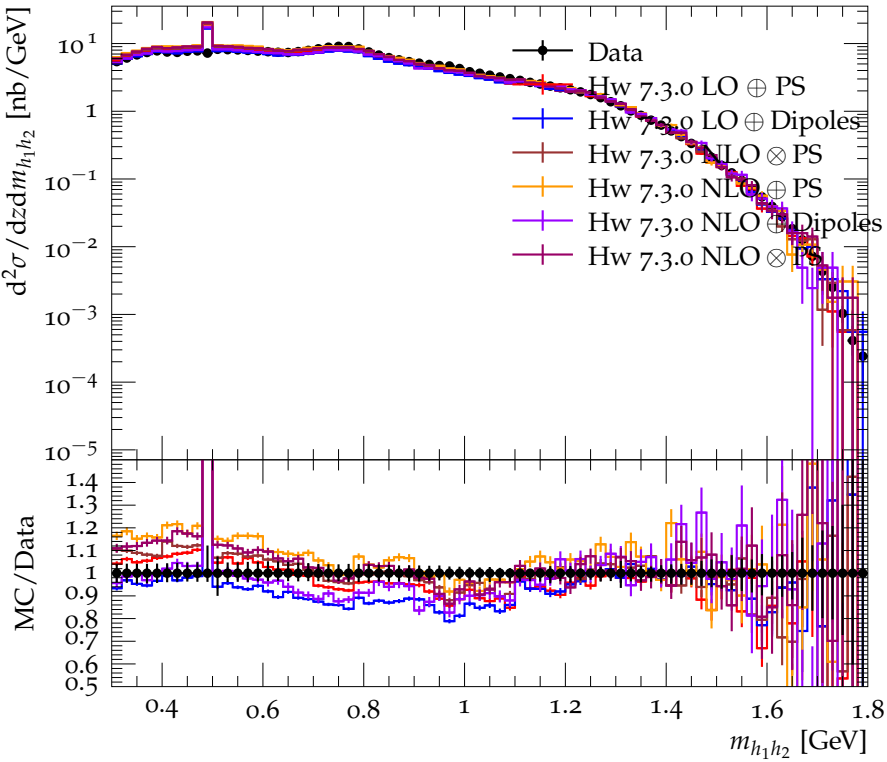
Differential cross section for \pi^+\pi^- ( 0.3 < z < 0.35 ) (strong)
