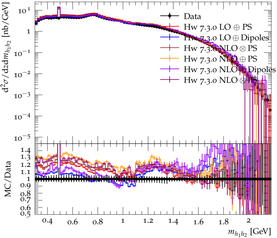
Differential cross section for \pi^+\pi^- ( 0.4 < z < 0.45 ) (strong)
