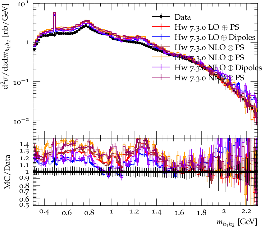
Differential cross section for \pi^+\pi^- ( 0.55 < z < 0.6 ) (strong)
