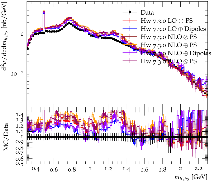
Differential cross section for \pi^+\pi^- ( 0.6 < z < 0.65 ) (strong)
