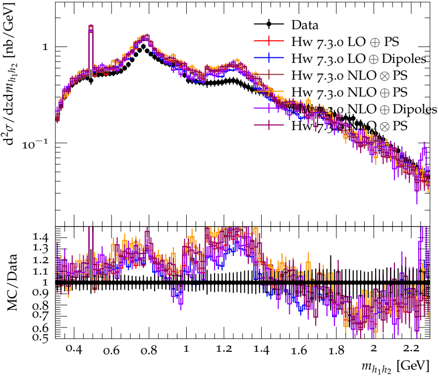
Differential cross section for \pi^+\pi^- ( 0.7 < z < 0.75 ) (strong)
